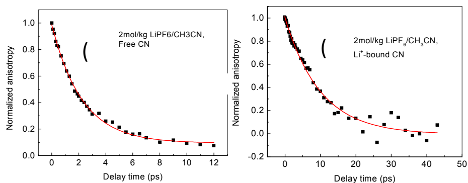
Fig.S6 Time dependent anisotropies of nitrile stretch of free \text{CH}_3\text{CN} (A) and \text{Li}^+ -bound \text{CH}_3\text{CN} (B) in a 2 mol/kg \text{LiPF}_6/\text{CH}_3\text{CN} solution. \text{Li}^+ -bound CN rotational time constant is 10.0 \pm 1\text{ps} , free CN rotational time constant is 2.2 \pm 0.2\text{ps} .
