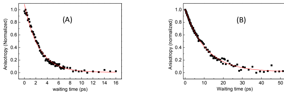
Fig.S4 Time dependent anisotropies of nitrile stretch of free \text{CH}_3\text{CN} (A) and \text{Li}^+ -bound \text{CH}_3\text{CN} (B) in a 2 mol/kg \text{LiBF}_4/\text{CH}_3\text{CN} solution. \text{Li}^+ -bound CN rotational time constant is 11 \pm 1 \text{ ps} , free CN rotational time constant is 2.5 \pm 0.2 \text{ ps} .
