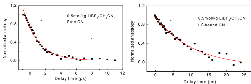
Fig.S3 Time dependent anisotropies of nitrile stretch of free CH 3 CN (A) and Li + -bound CH 3 CN (B) in a 0.5 mol/kg LiBF 4 /CH 3 CN solution. Li + -bound CN rotational time constant is 10 \pm 1 ps, free CN rotational time constant is 2.0 \pm 0.2 ps
