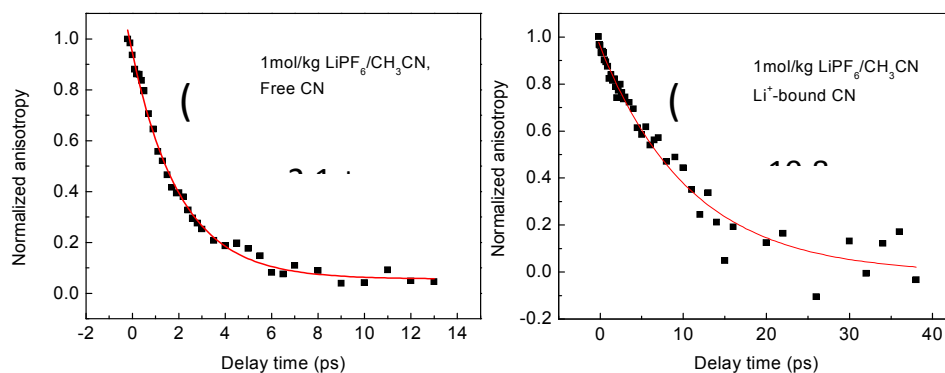
Fig.S5 Time dependent anisotropies of nitrile stretch of free \text{CH}_3\text{CN} (A) and \text{Li}^+ -bound \text{CH}_3\text{CN} (B) in a 1 mol/kg \text{LiPF}_6/\text{CH}_3\text{CN} solution. \text{Li}^+ -bound CN rotational time constant is 10.8 \pm 1 \text{ ps} , free CN rotational time constant is 2.1 \pm 0.2 \text{ ps}
