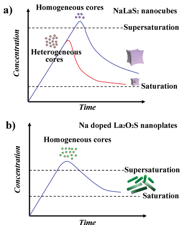
Figure 6. LaMer schemes of (a) \text{NaLaS}_2 NCs and (b) Na-doped \text{La}_2\text{O}_2\text{S} NCs.
