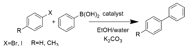
Figure 7. Suzuki cross-coupling reaction between aryl halide (iodobenzene, bromobenzene, or 4-bromotoluene) and phenylboronic acid used in the present work was utilized to evaluate catalytic activities of nanocatalysts.
