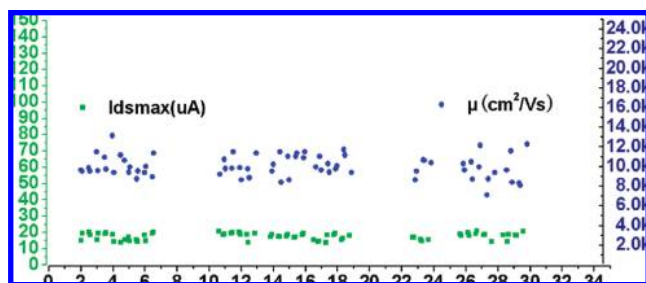
Figure 5. The electrical properties along a 3 cm long SWNT with a diameter of 1.36 nm. Green square: the I_{dsmax} ( V_{ds} = 10 V, V_{gs} = -20 V) of the SWNT devices fabricated along this SWNT with a channel length of 2 \mu m and 200 nm wide Cr (10 nm)/Pt (50 nm) as source and drain pads. Blue circle: the mobility of those SWNT devices ( V_{ds} = 1 V, V_{gs} = -20 V); the effects of the contact are subtracted.
